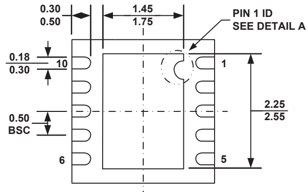
QFN10 (3mm x 3mm)
