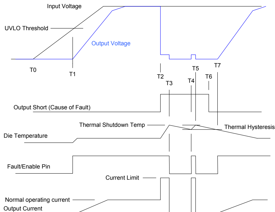
Figure 3—Thermal Protection in Short Condition
