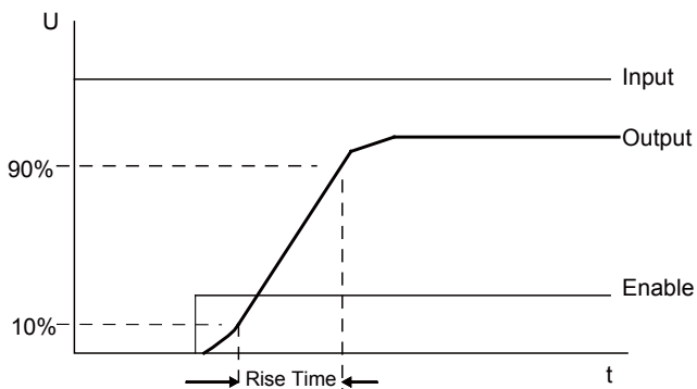
Figure 2—Rise Time
