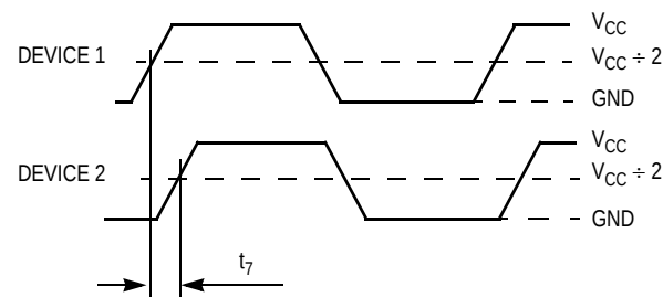
Figure 4. Device-to-Device Skew
