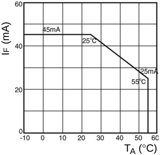
Forward Current Reduction Curve
