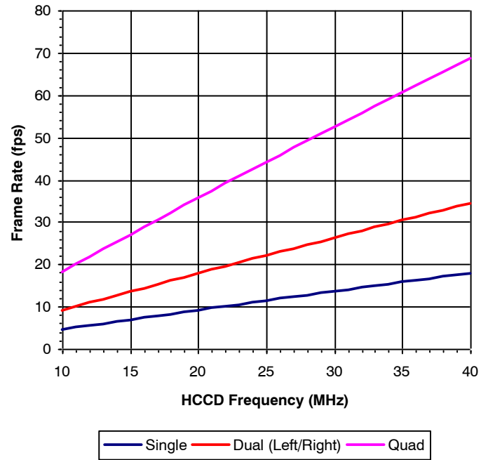
Figure 12. Frame Rates
