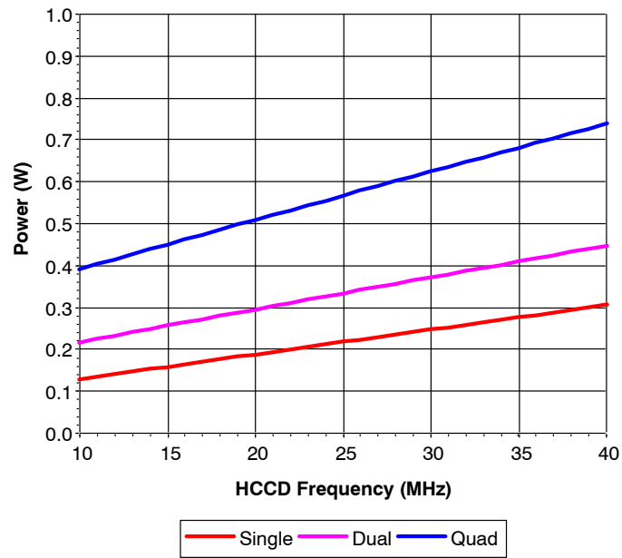
Figure 11. Power
