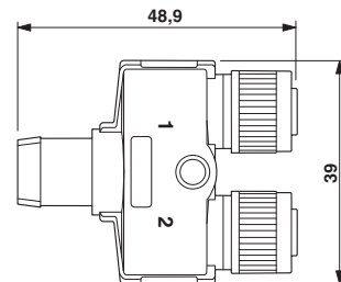
Y distributor, 2 x socket M12 x 1
