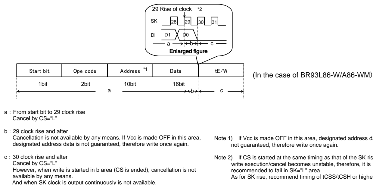
Fig.67 WRITE, WRAL cancel available timing
