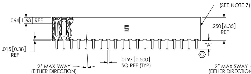
FIG 1 SQT-120-01-XX-6 SHOWN
