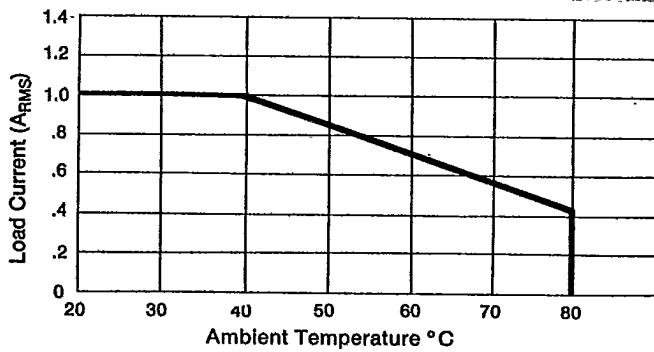
Figure 1. Derating Curve
