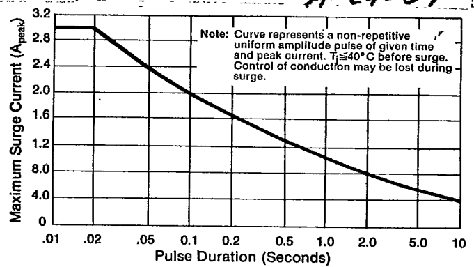
Figure 2. Maximum Allowable Surge
