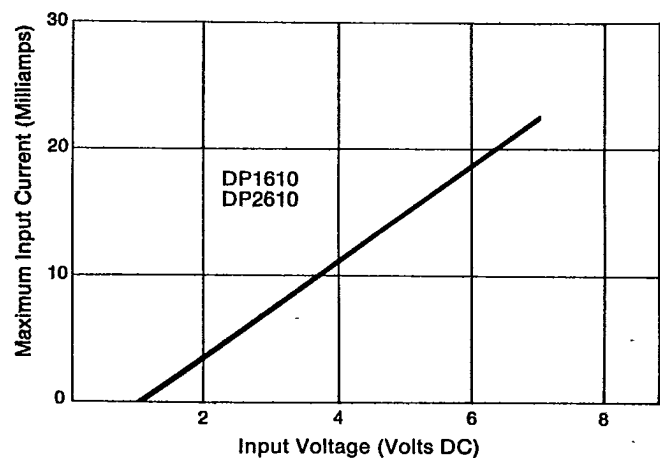
Figure 4. Input Characteristics (Voltage Controlled)
