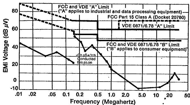
Figure 5. Conducted Electromagnetic Interference
