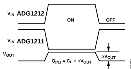
Figure 25. Charge Injection
