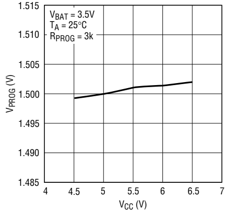
PROG Pin Voltage vs V_{\text{CC}} Constant Current Mode
