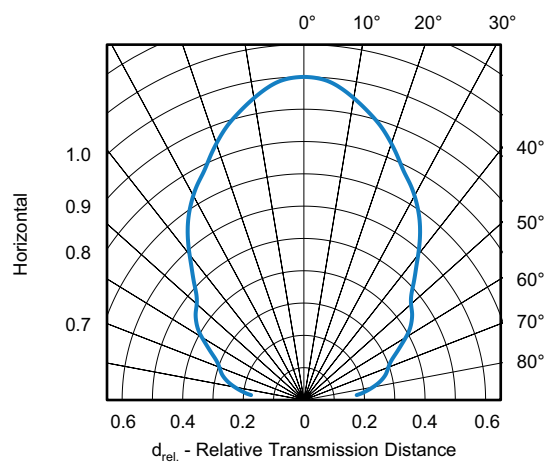
Fig. 11 - Horizontal Directivity
