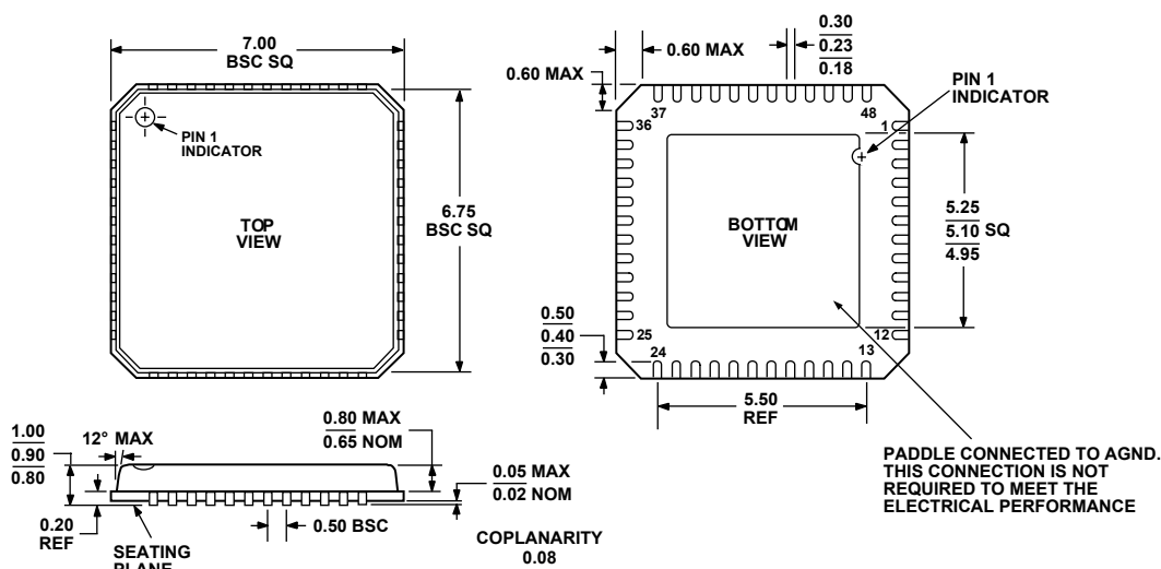
Figure 47. 48-Lead Frame Chip Scale Package (LFCSP) (CP-48)
