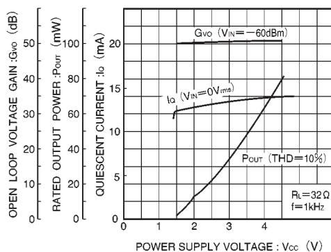
Fig. 8 Open loop voltage gain/quiescent current/rated output power vs. power supply voltage
