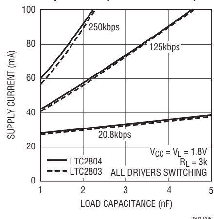
Supply Current vs Load Capacitance (Dual Transceiver)
