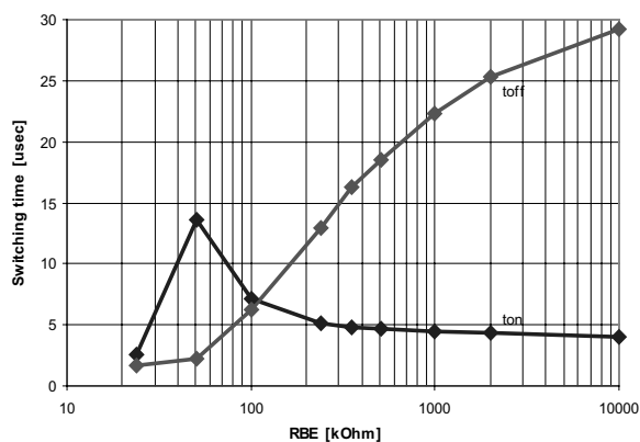
Figure 21. Switching time vs. R_{BE} , I_F = 10mA
