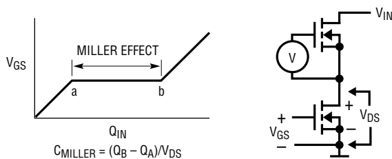
Figure 9. Gate Charge Characteristic
