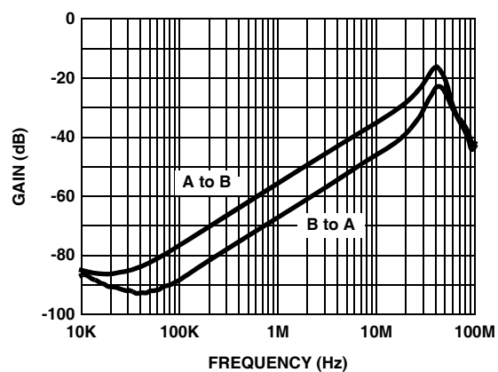
FIGURE 14. CHANNEL SEPARATION
