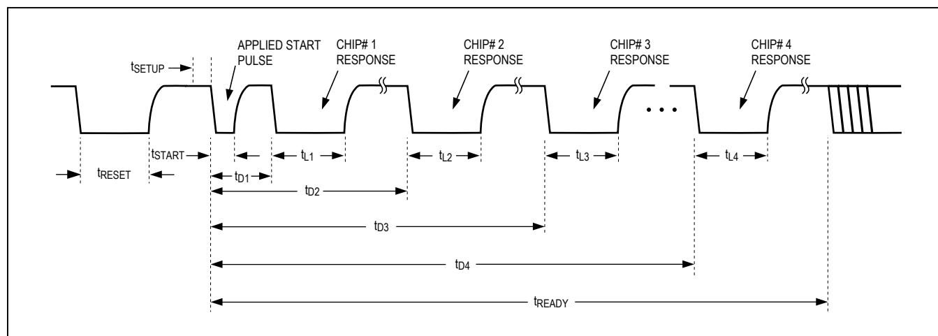
Figure 1. Timing Diagram
