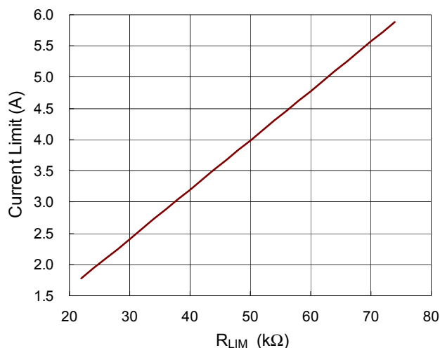
Figure 4. Channel 1 Current Limit vs. R_{LIM}
