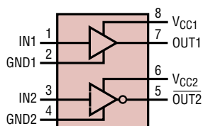
LTC1693-2 TOPSIDE NONINVERTING DRIVER AND BOTTOM SIDE INVERTING DRIVER
