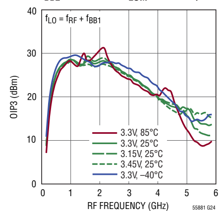
Output IP3 vs RF Frequency for High Side LO Injection ( f_{BB1} = 140MHz , f_{BB2} = 141MHz , P_{LOM} = 10dBm )
