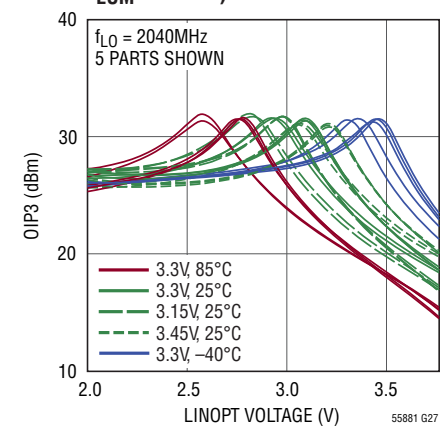
Output IP3 vs LINOPT Voltage ( f_{RF1} = 1899MHz , f_{RF2} = 1900MHz , P_{LOM} = 0dBm )
