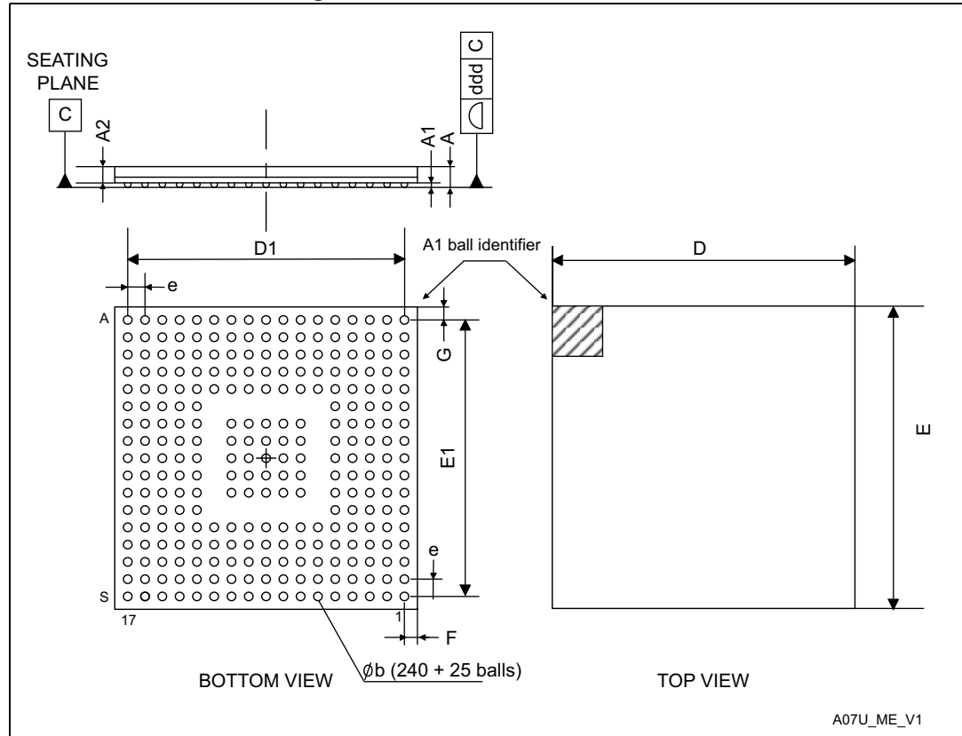
Figure 124. TFBGA240+25 - Outline
