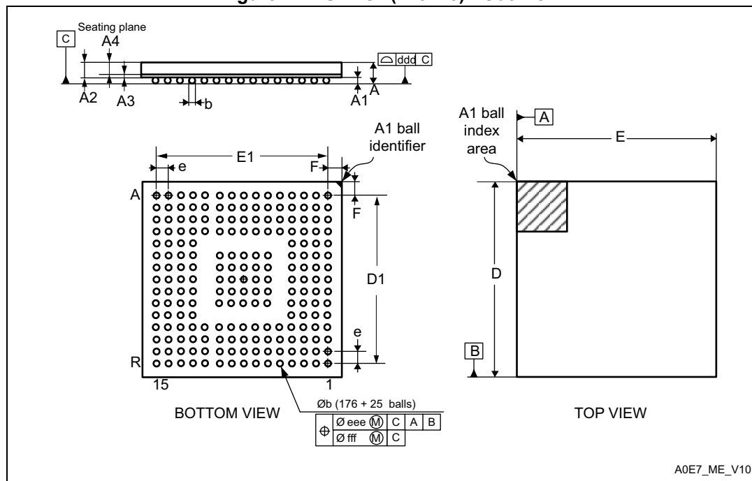
Figure 122. UFBGA(176+25) - Outline
