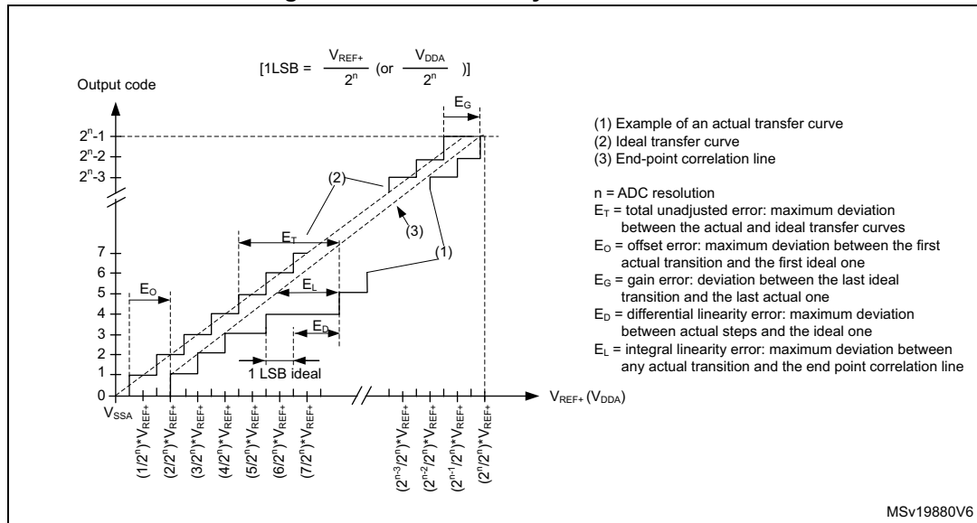
Figure 88. ADC accuracy characteristics
