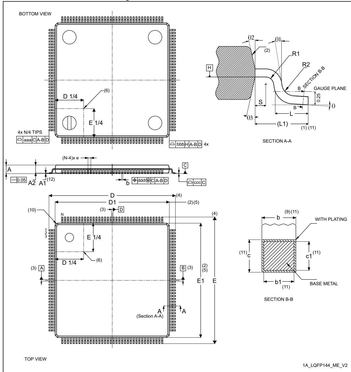
Figure 118. LQFP144 - Outline (15)
