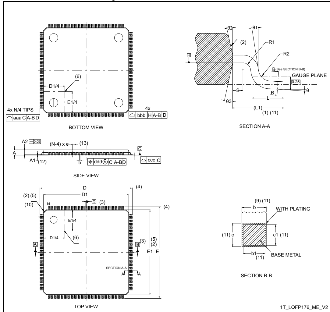
Figure 120. LQFP176 - Outline (15)
