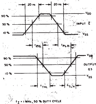
Fig. 17 - CD4555B \bar{E} input to Q3 output dynamic signal waveforms.
