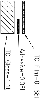
DETAIL-A
