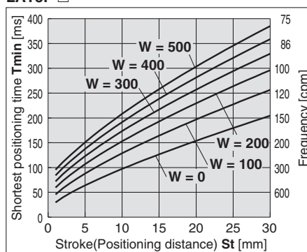
Fig. 3 Shortest Positioning Time (Guide): T_{min} [ms]
