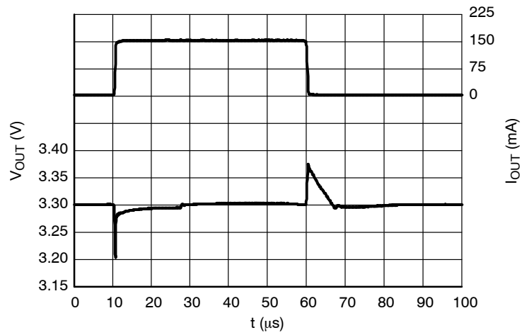
Figure 46. Load Transients, 3.3 V Version, I_{OUT} = 1 - 150 \text{ mA} , t_R = t_F = 0.5 \mu\text{s} , V_{IN} = 4.3 \text{ V}
