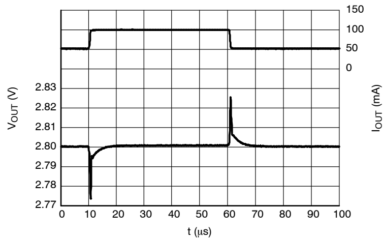
Figure 42. Load Transients, 3.3 V Version, I_{OUT} = 50 - 100 mA, t_R = t_F = 0.5 \mu s, V_{IN} = 4.3 V
