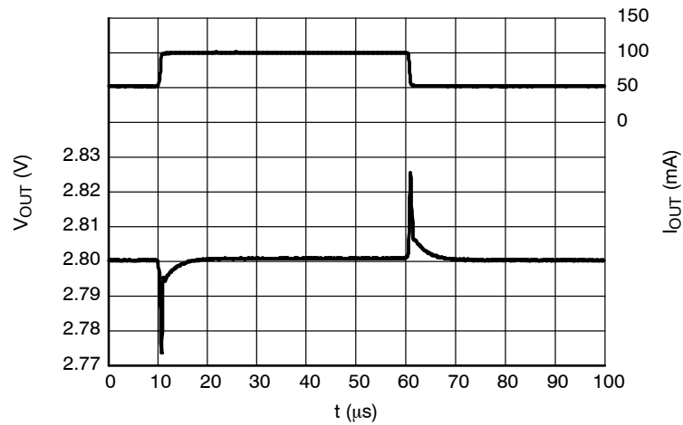
Figure 41. Load Transients, 2.8 V Version, I_{OUT} = 50 - 100 mA, t_R = t_F = 0.5 \mu s, V_{IN} = 3.8 V
