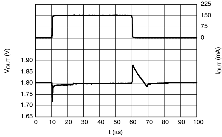
Figure 44. Load Transients, 1.8 V Version, I_{OUT} = 1 - 150 \text{ mA} , t_R = t_F = 0.5 \mu\text{s} , V_{IN} = 2.8 \text{ V}
