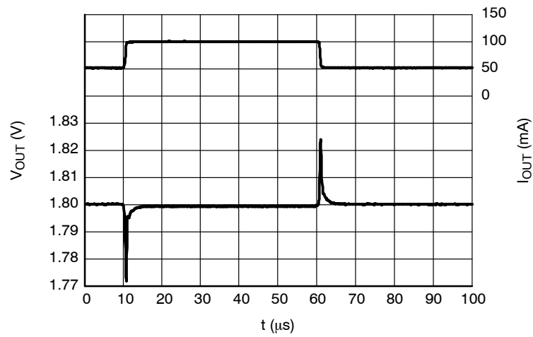
Figure 40. Load Transients, 1.8 V Version, I_{OUT} = 50 - 100 mA, t_R = t_F = 0.5 \mu s, V_{IN} = 2.8 V
