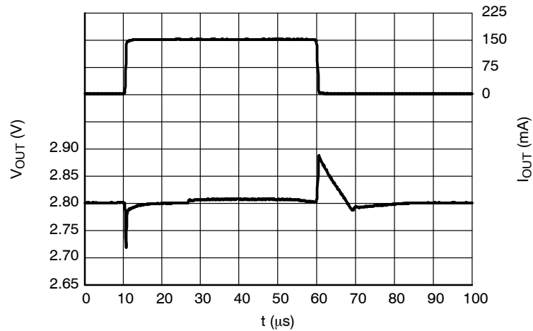
Figure 45. Load Transients, 2.8 V Version, I_{OUT} = 1 - 150 \text{ mA} , t_R = t_F = 0.5 \mu\text{s} , V_{IN} = 3.8 \text{ V}
