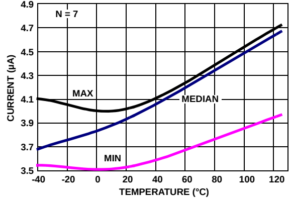
FIGURE 26. ISL28276 SUPPLY CURRENT vs TEMPERATURE, V_+ , V_- = \pm 2.5V DISABLED, R_L = \infty
