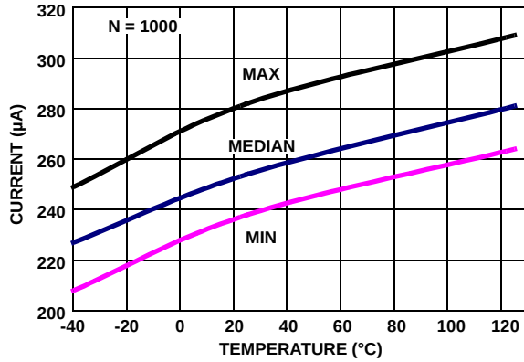
FIGURE 25. ISL28476 SUPPLY CURRENT vs TEMPERATURE, V_+ , V_- = \pm 2.5V ENABLED, R_L = \infty
