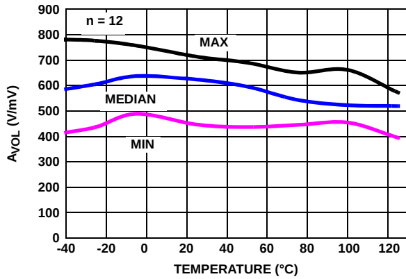
FIGURE 43. ISL28176 A_{VOL} , R_L = 100k , V_S = \pm 2.5V , V_O = \pm 2V
