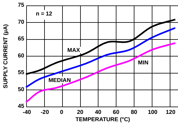
FIGURE 23. ISL28176 SUPPLY CURRENT vs TEMPERATURE V_S = \pm 2.5V ENABLED, R_L = \text{INF}
