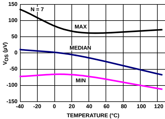
FIGURE 29. ISL28276 V_{OS} vs TEMPERATURE, V_{IN} = 0V , V_+ , V_- = \pm 2.5V
