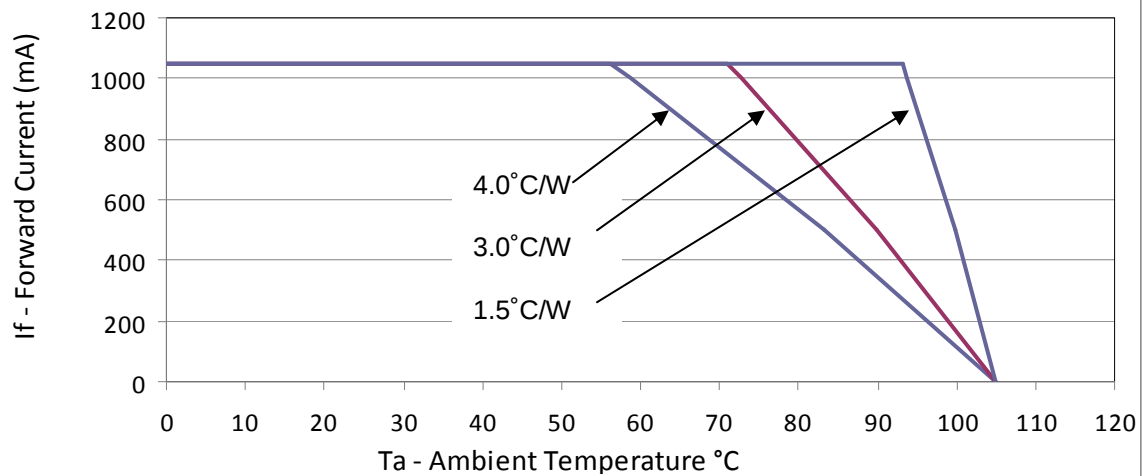
Figure 27: Derating Curve for BXRA-C1202, 1050 mA Drive Current
