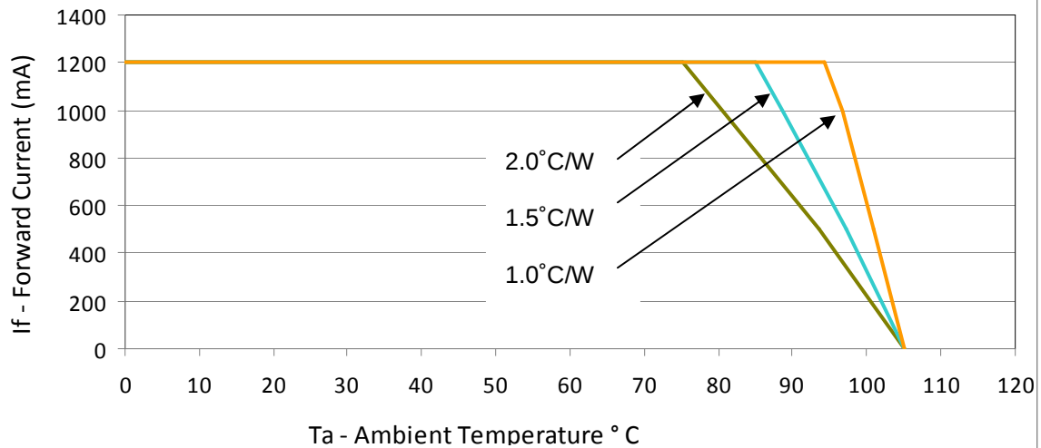
Figure 28: Derating Curve for BXRA-W1202, 1200 mA Drive Current
