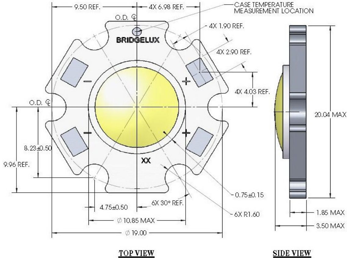
Figure 1: Drawing for 400 lumen product options (part numbers BXRA-C0402, BXRA-W0401 and BXRA-W0402).
