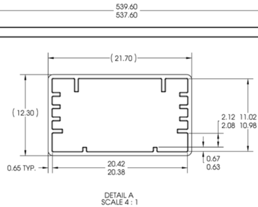
Figure 37: Tube Design for Hexagonal Star Products
