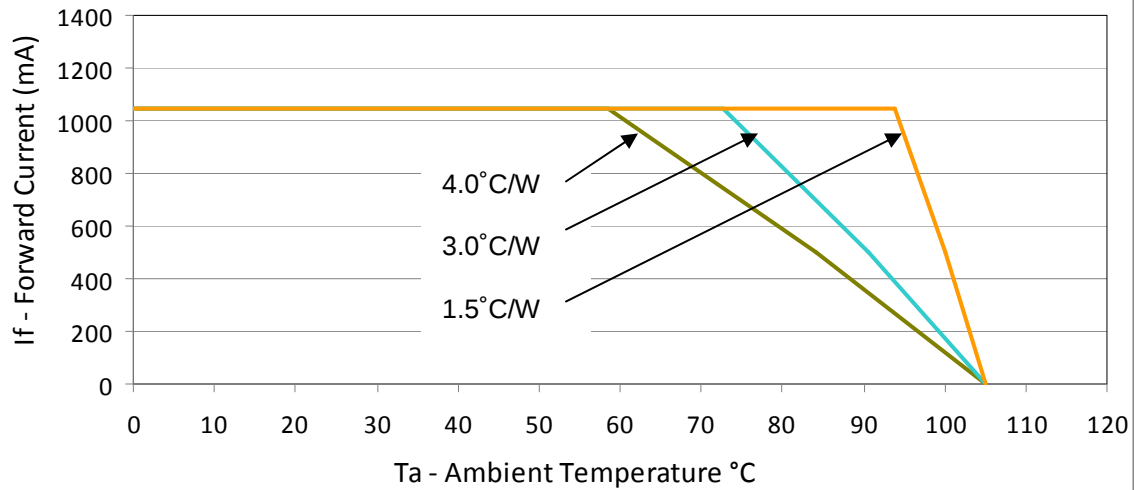
Figure 26: Derating Curve for BXRA-W0802, 1050mA Drive Current
