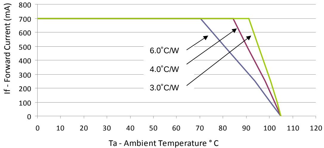
Figure 24: Derating Curve for BXRA-W0402, 700mA Drive Current
