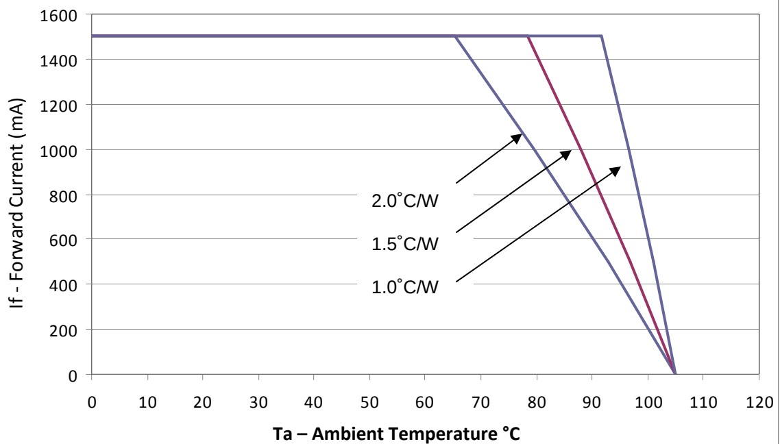
Figure 29: Derating Curve for BXRA-C2002, 1500 mA Drive Current
