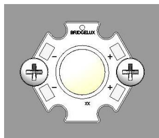
Figure 33: Recommended Mounting Locations for Hexagonal Star Products
