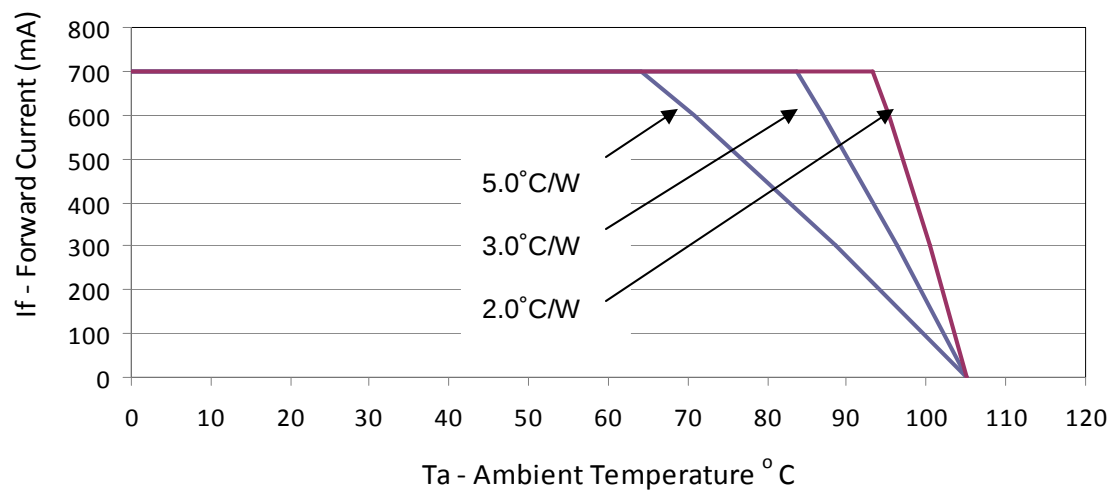
Figure 25: Derating Curve for BXRA-C0802, 700mA Drive Current
