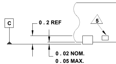
DETAIL "X"
