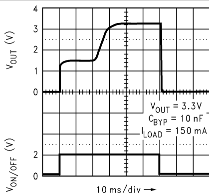
Figure 7-28. Turn-On Time (Legacy Chip)
