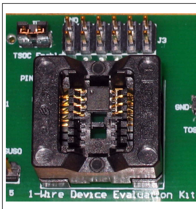
Figure 4. TSOC Package Insertion
