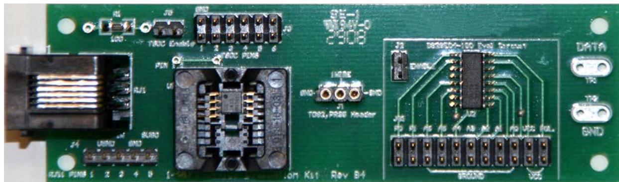
Figure 1. DS9090 EV Kit Board Layout
