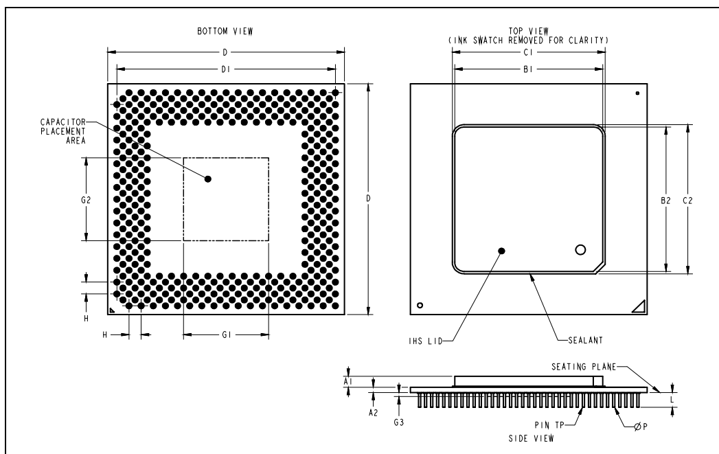
Figure 24. Package Dimensions (FC-PGA2 Package)
