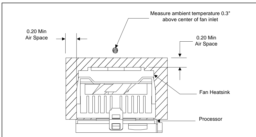
Figure 40. Volumetric Keepout Requirements for The Boxed Fan Heatsink
