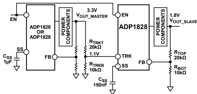
Figure 43. Example of a Coincident Tracking Circuit
