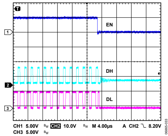
Figure 33. EN, Shutdown
