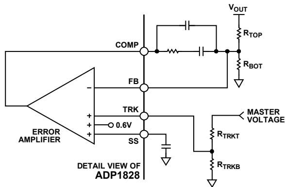
Figure 42. Voltage Tracking
