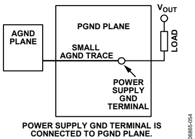
Figure 53. Proper Grounding Technique for a Heavy Load
