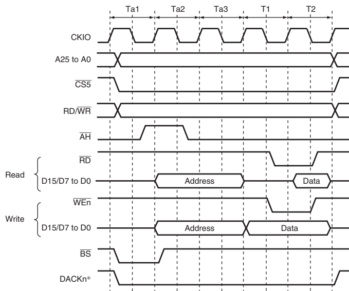
Figure 9.10 (1) Access Timing for MPX Space (Address Cycle No Wait, Data Cycle No Wait)
