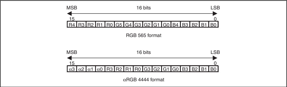
Figure 28.18 Bus Format
