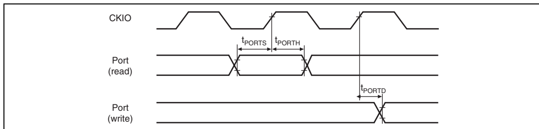
Figure 37.77 General I/O Ports Timing
