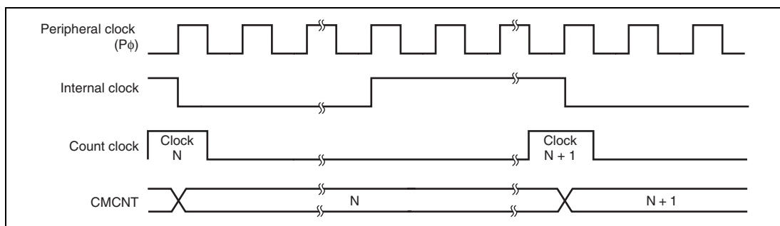
Figure 12.3 Count Timing
