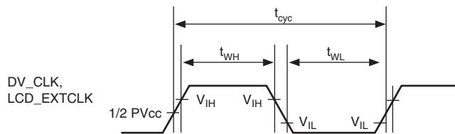
Figure 37.72 DV_CLK and LCD_EXTCLK Clock Input Timing
