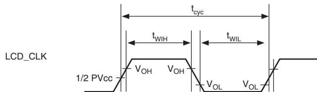
Figure 37.73 LCD_CLK Clock Output Timing
