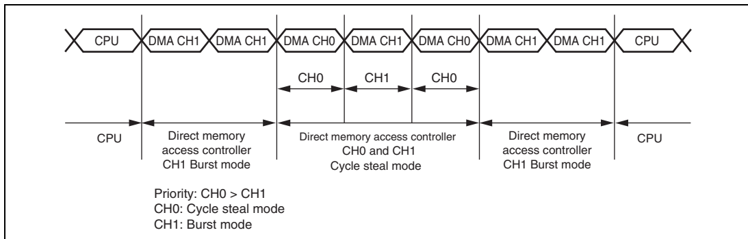
Figure 10.10 Bus State when Multiple Channels are Operating
