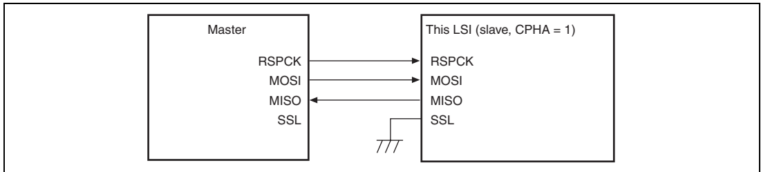
Figure 16.4 Master/Slave Configuration Example (This LSI = Slave, CPHA = 1)
