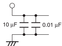
Figure 25.8 Example of Analog Input Protection Circuit
