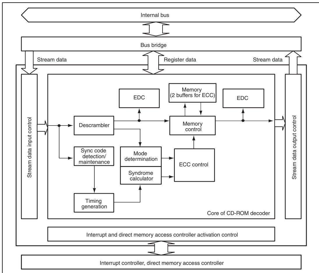
Figure 24.2 Block Diagram
