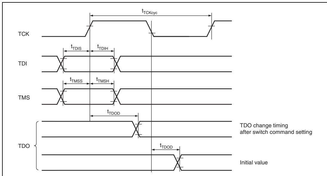
Figure 37.79 Data Transfer Timing
