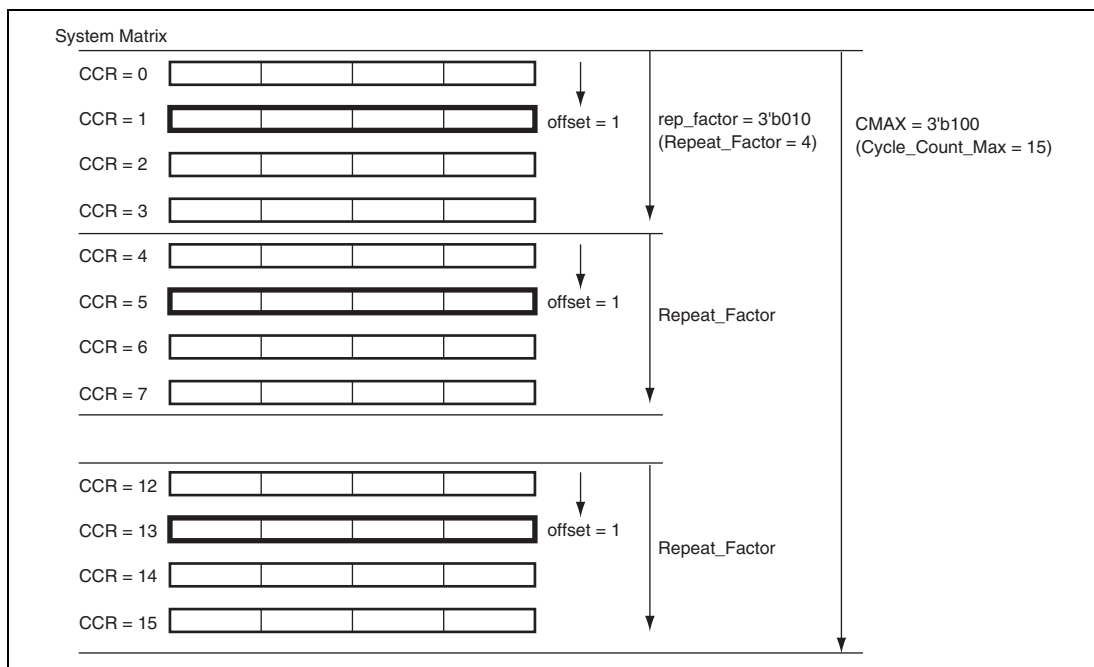
Figure 21.8 System Matrix
