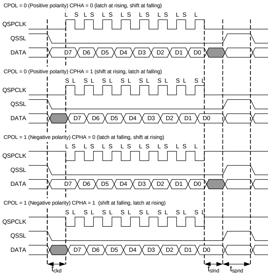
Figure 17.1 SPI Clock Setting and Transfer Timing
