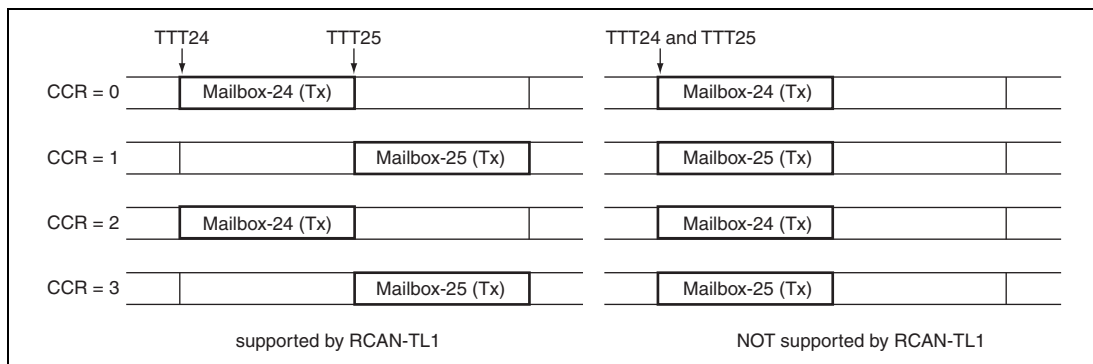
Figure 21.18 Limitation on Tx-Trigger Time
