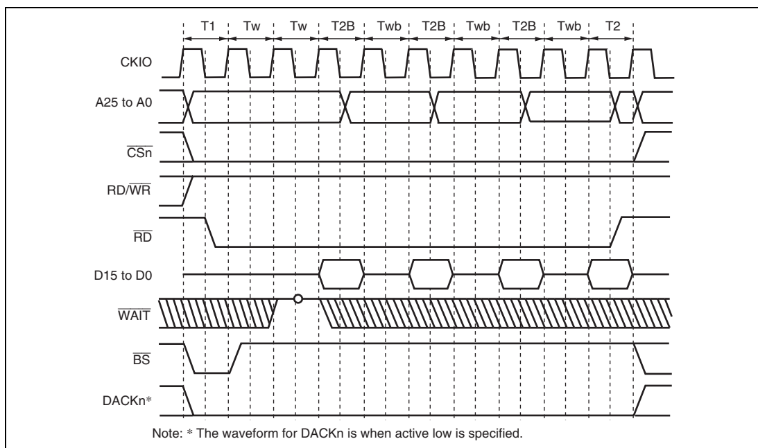
Figure 9.31 Burst ROM Access Timing (Clocked Asynchronous)
