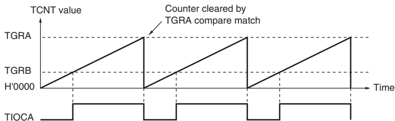
Figure 11.26 Example of PWM Mode Operation (1)
