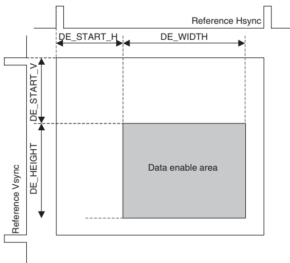
Figure 28.23 DE Area Settings
