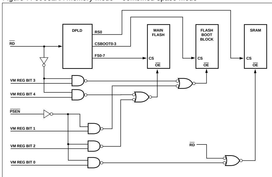
Figure 7. 80C51XA Memory Mode – Combined Space Mode
