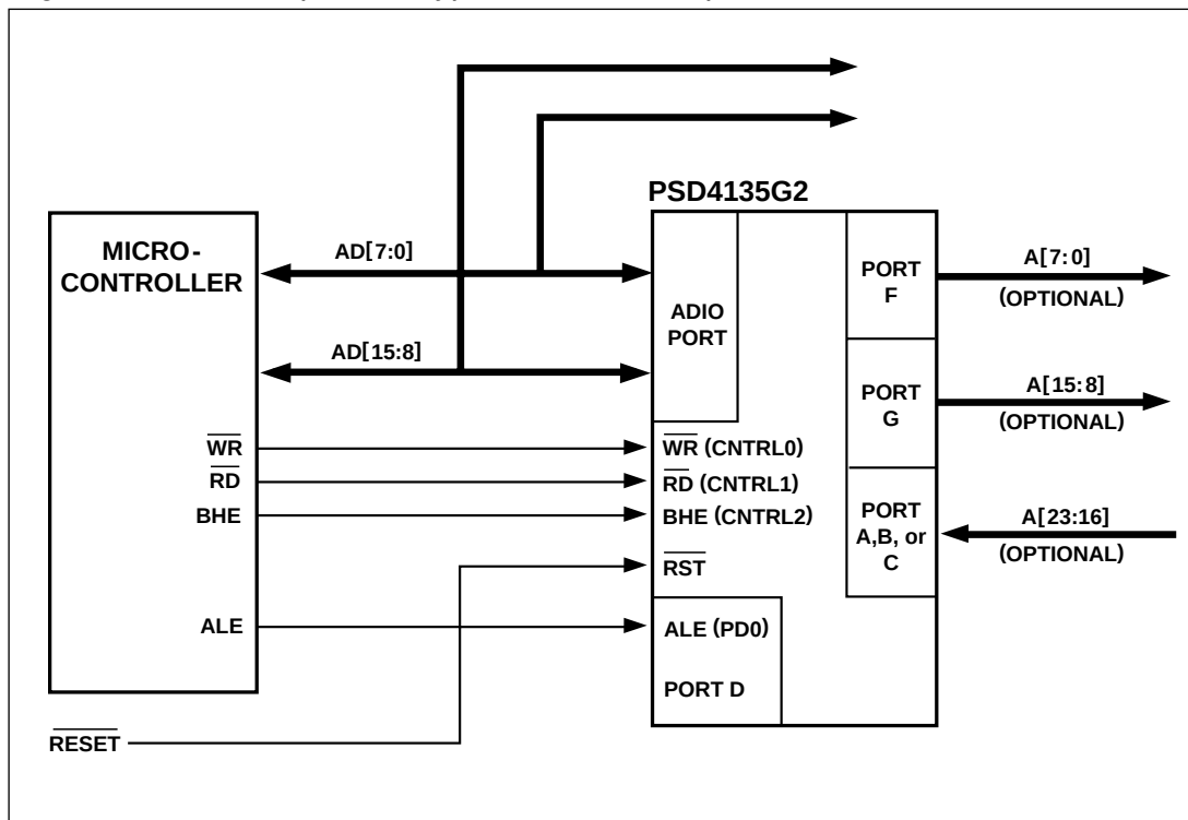
Figure 12. An Example of a Typical 16-Bit Multiplexed Bus Interface
