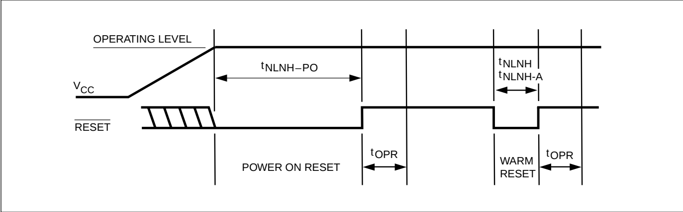
Figure 32. Reset Timing
