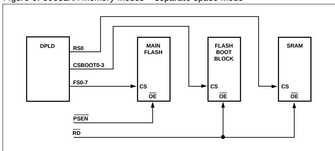
Figure 6. 80C51XA Memory Modes – Separate Space Mode
