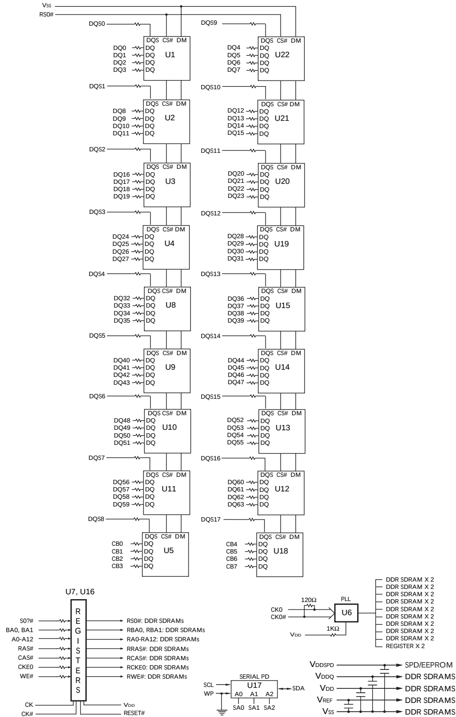
Figure 3: Functional Block Diagram – Standard Low-Profile PCB
