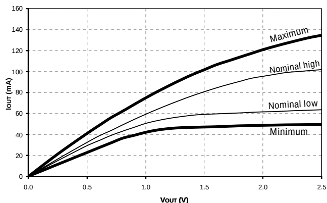
Figure 10: Pull-Down
