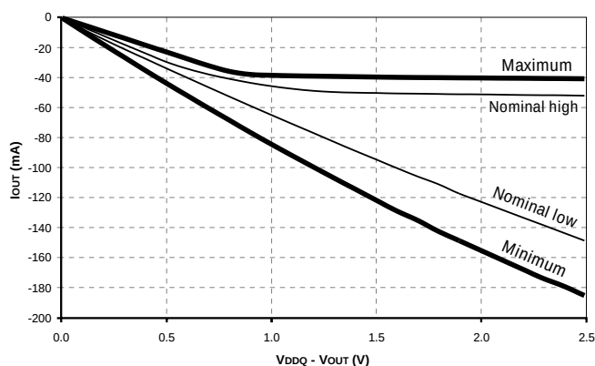
Figure 11: Pull-Up
