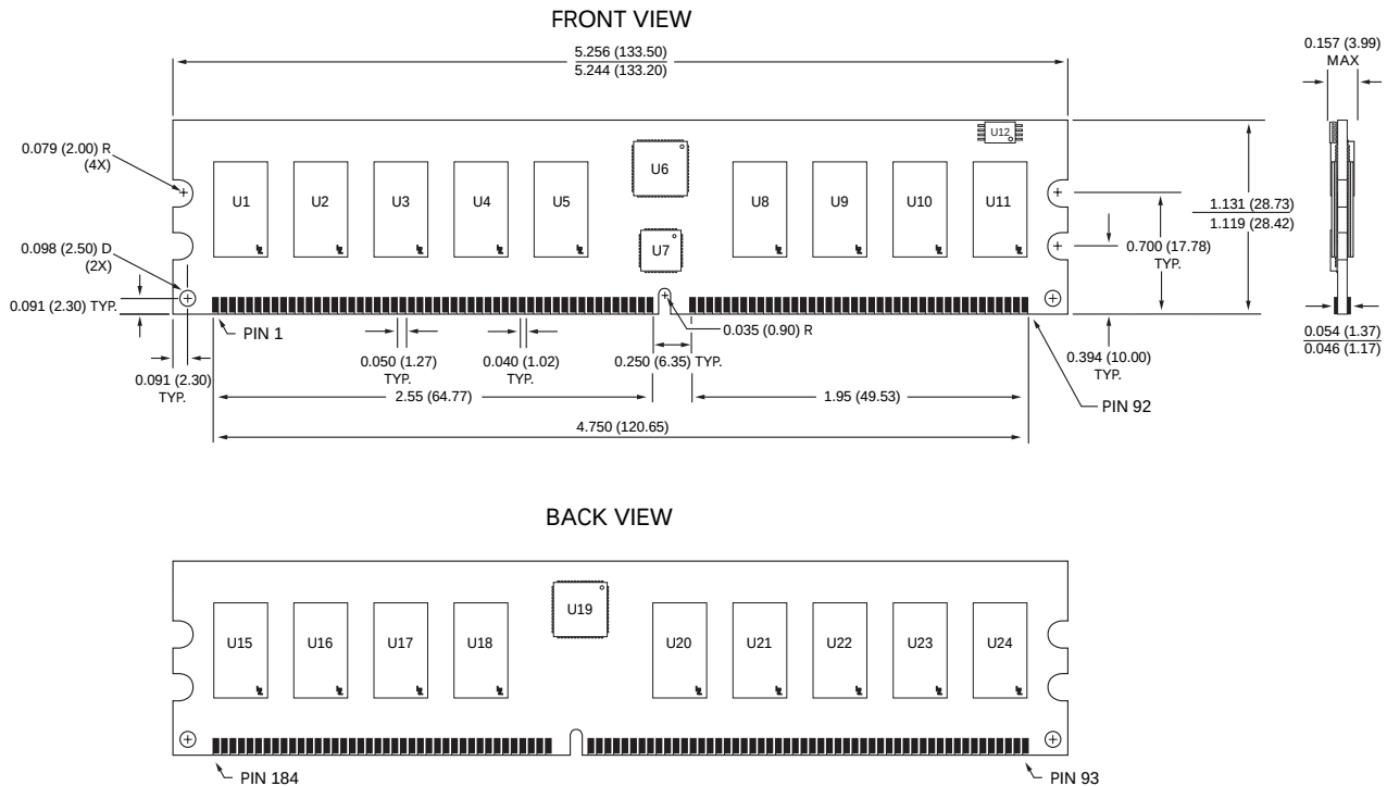
Figure 19: 184-Pin DIMM Dimensions – Alternate Low-Profile PCB
