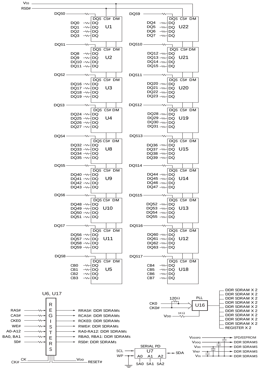
Figure 5: Functional Block Diagram – Very Low-Profile PCB
