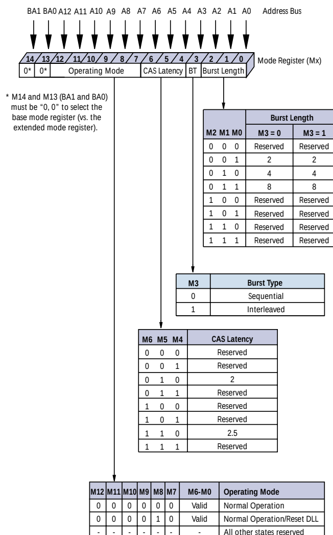
Figure 6: Mode Register Definition Diagram
