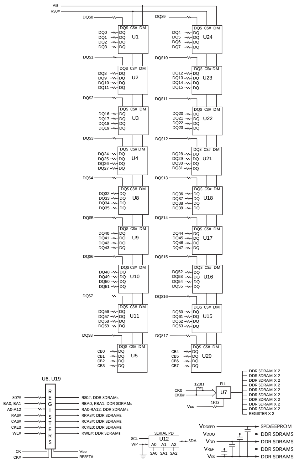
Figure 4: Functional Block Diagram – Alternate Low-Profile PCB
