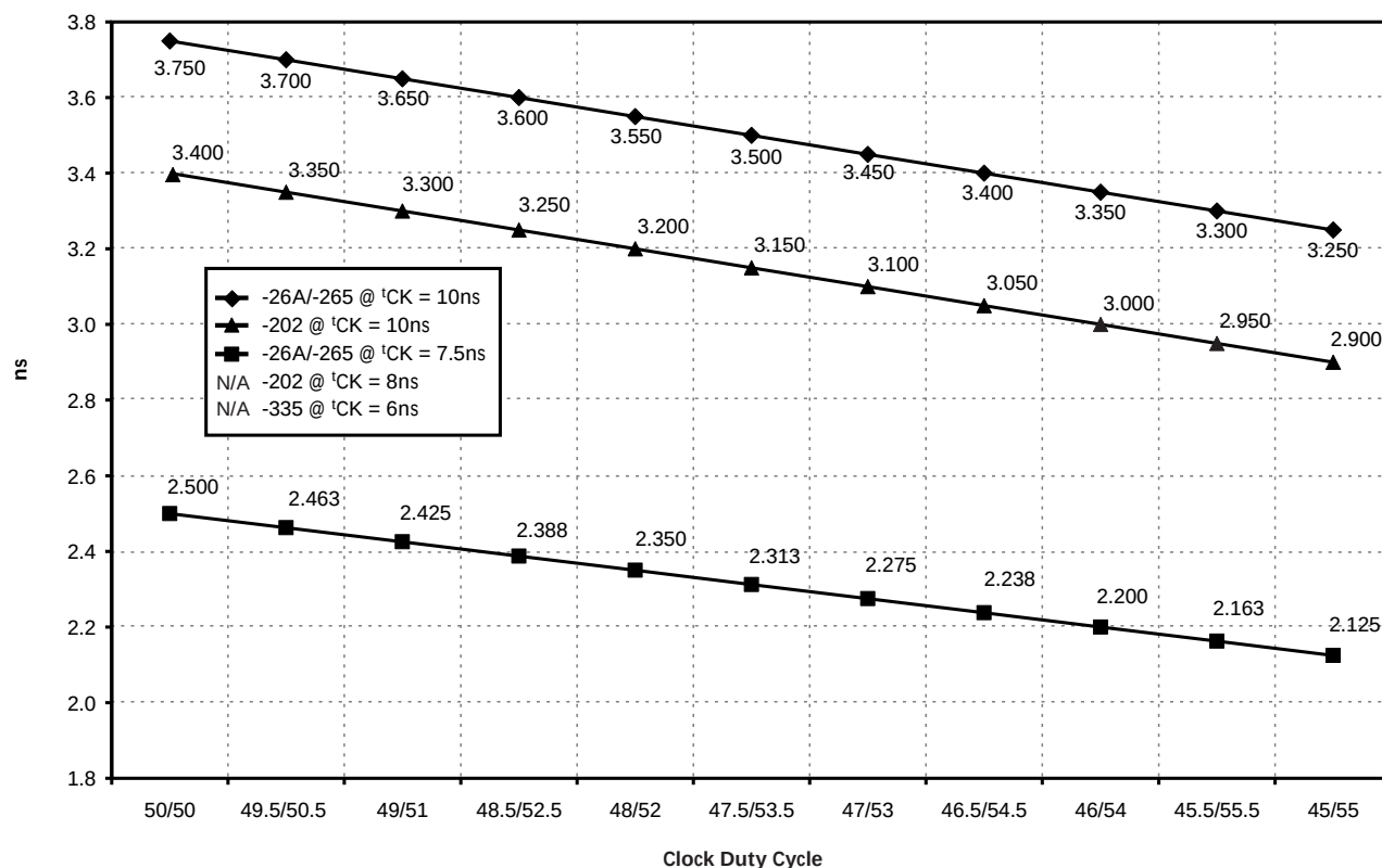
Figure 9: Derating Data Valid Window ( t_{QH} - t_{DQSQ} )
