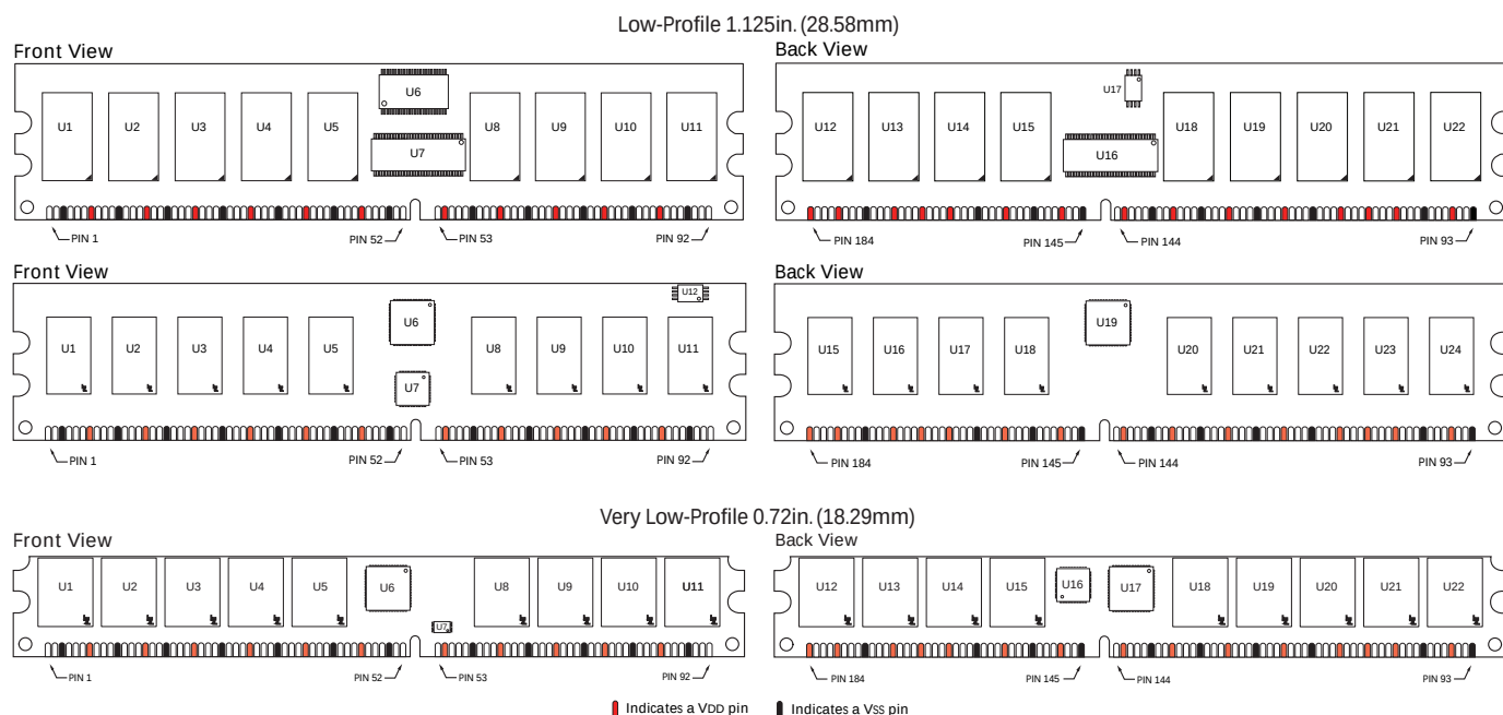
Figure 2: Pin Locations
