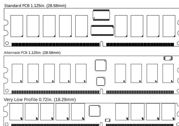
Figure 1: 184-Pin DIMM (MO-206)
