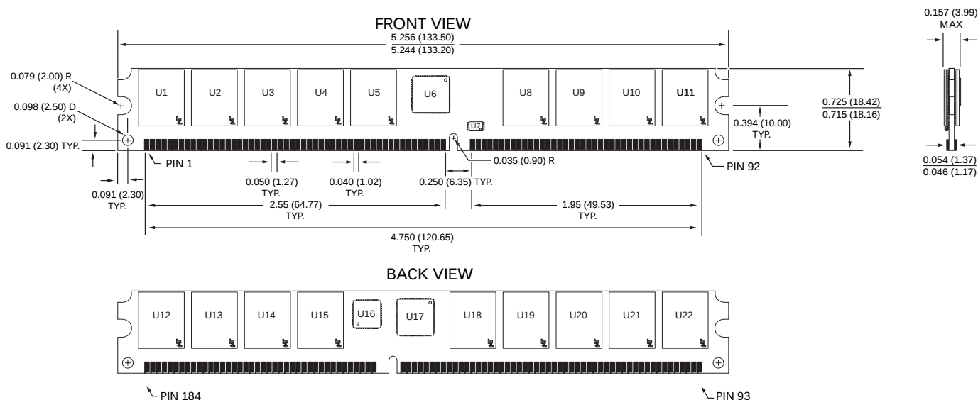
Figure 20: 184-Pin DIMM Dimensions – Very Low-Profile PCB
