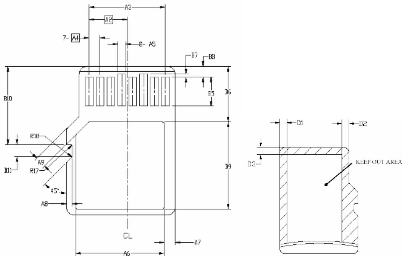
Figure 2. microSD Bottom View and Keep Out Area
