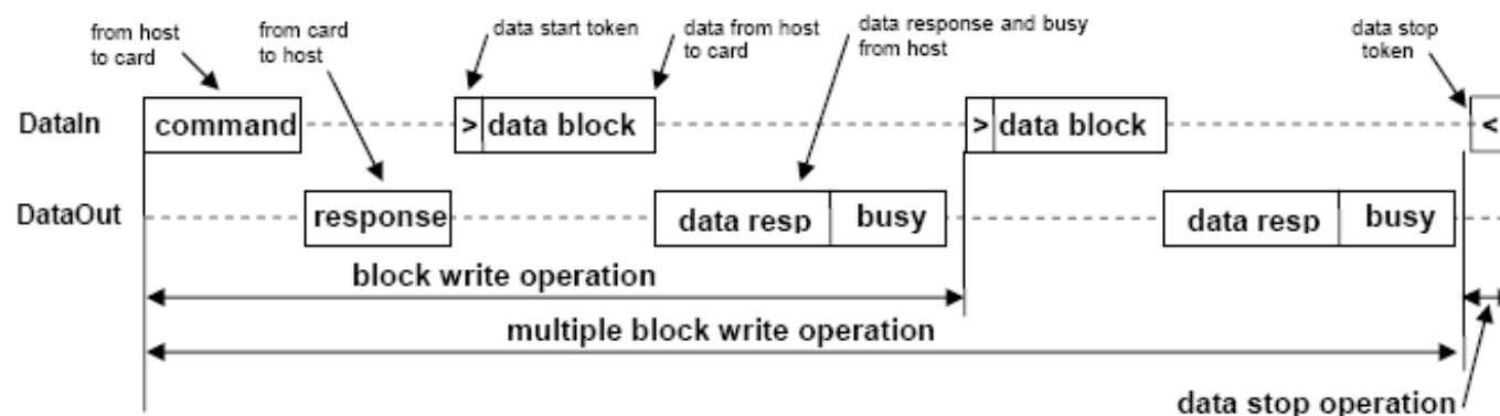
Figure 18. Write Operation
