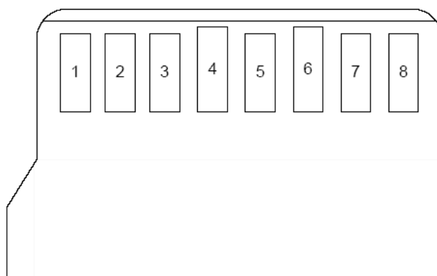
Figure 7. microSD Contacts
