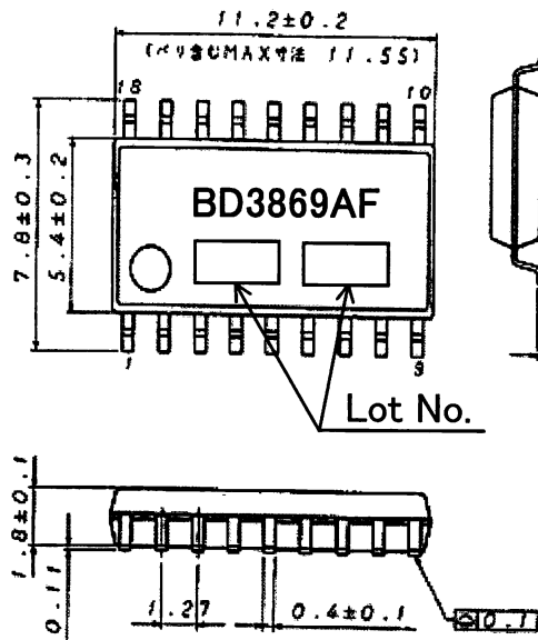
SOP-18 (Unit : mm)
