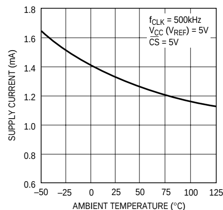
LTC1091 Supply Current vs Temperature
