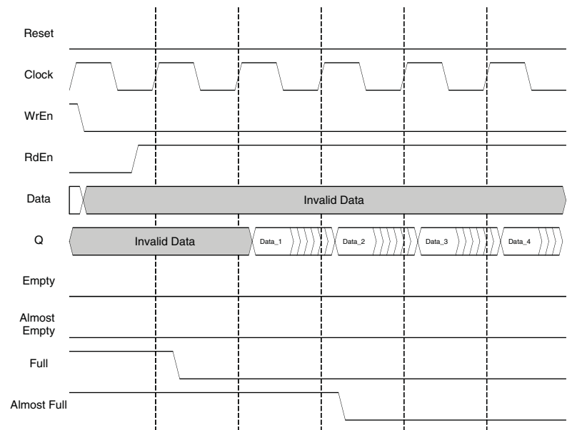
Figure 11-28. FIFO with Output Registers, End of Data Read Cycle
