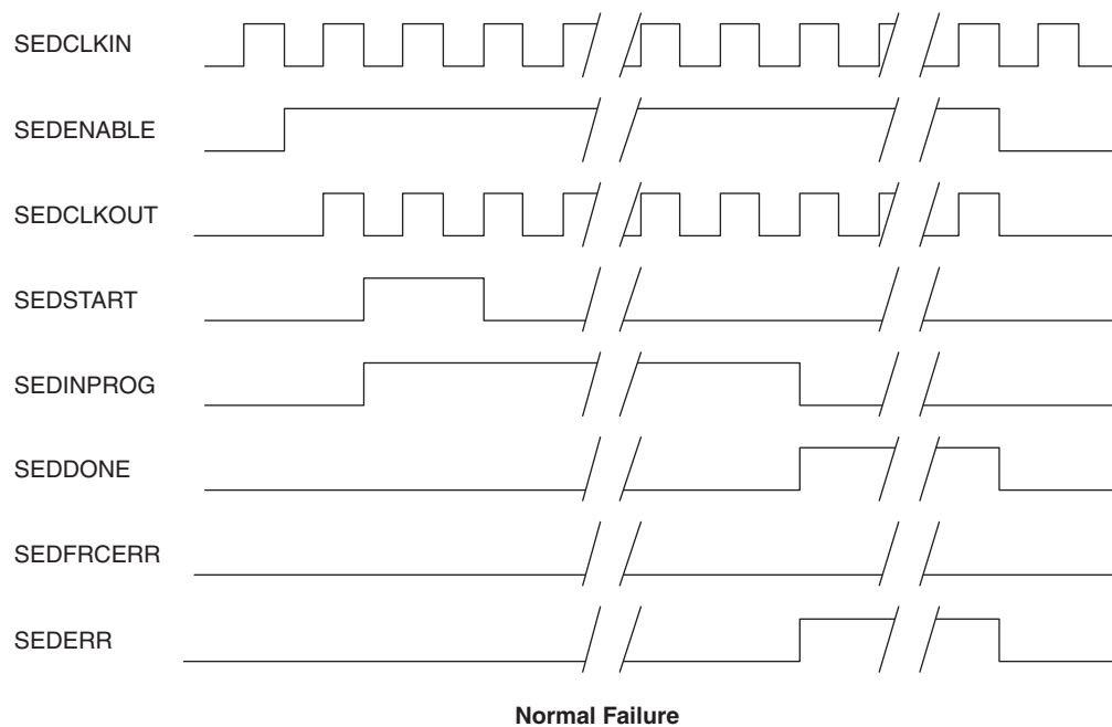
Figure 17-3. Timing Diagram
