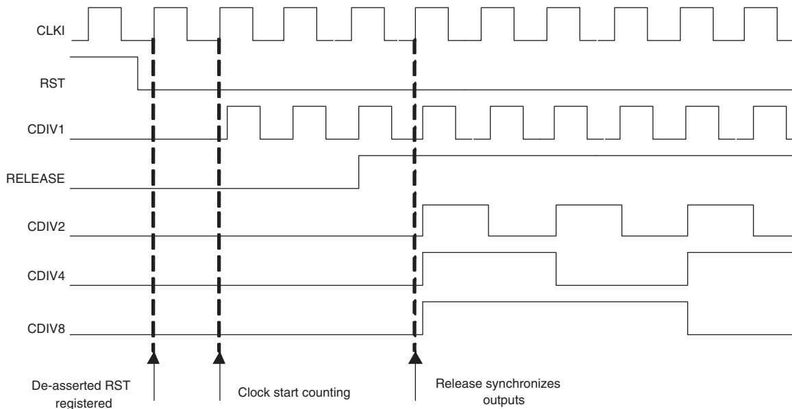
Figure 10-24. CLKDIV Release Behavior
