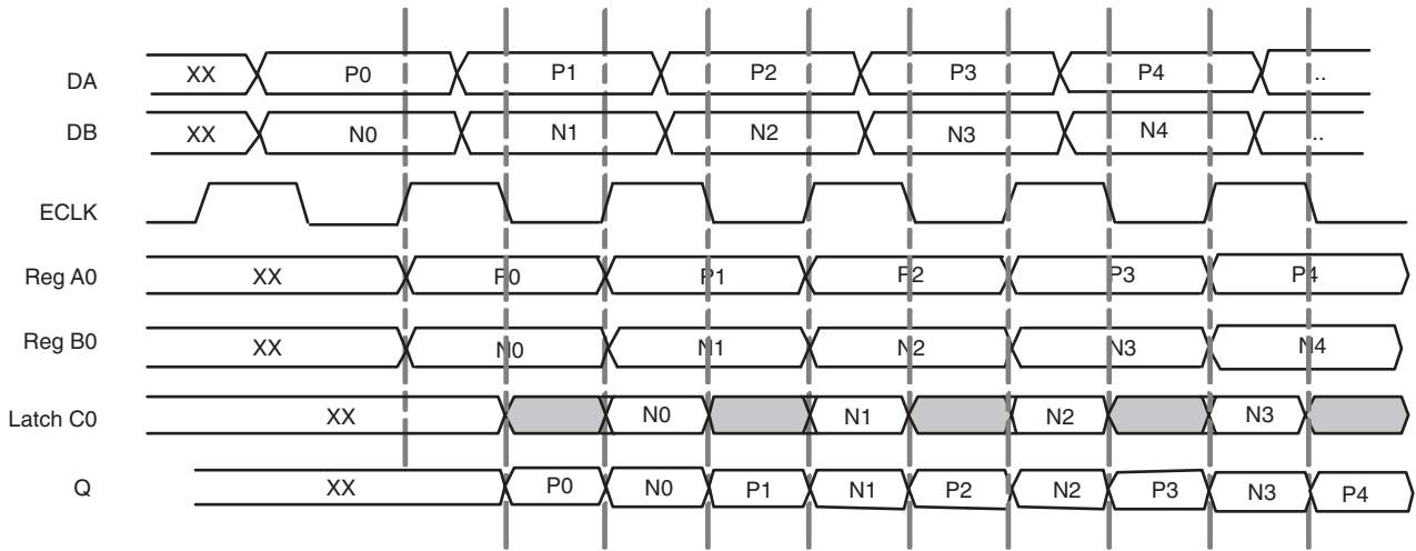
Figure 12-37. ODDRXC Waveform
