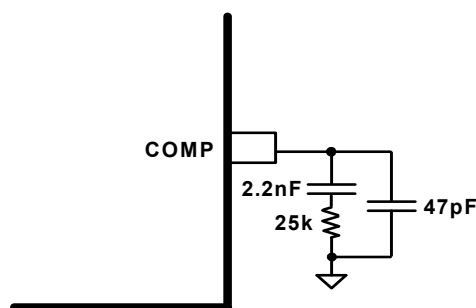
FIGURE 19. COMPENSATION NETWORK
