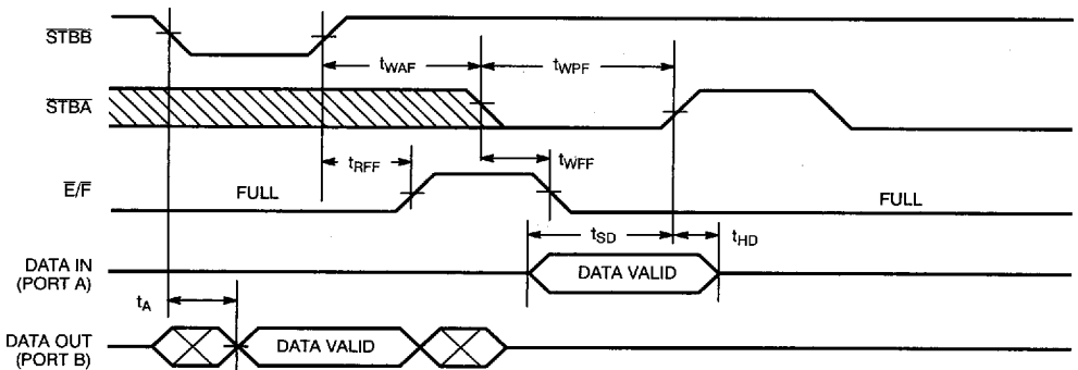
Empty/Full Flag and Write Bubble-Through Mode Timing Diagram [11]
