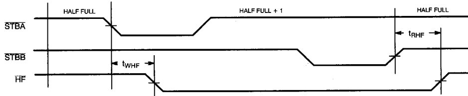
Half-Full Flag Timing Diagram [11]
