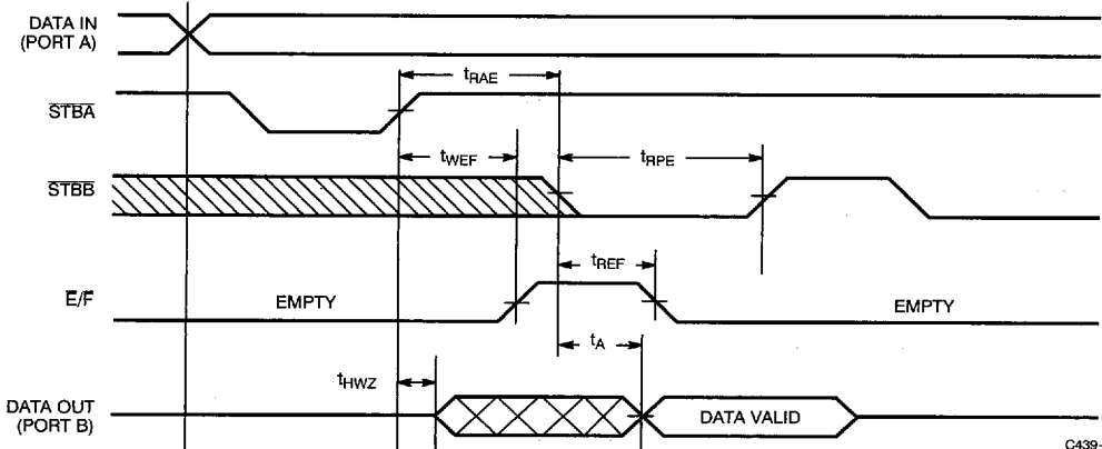
Empty/Full Flag and Write Bubble-Through Mode Timing Diagram [11]
