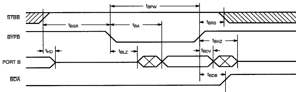
Registered Bypass Read Timing Diagram [12]
