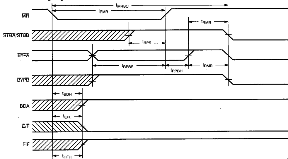
Half-Full Flag Timing Diagram [11]
