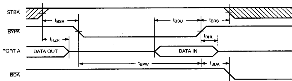
Registered Bypass Write Timing Diagram [13]
