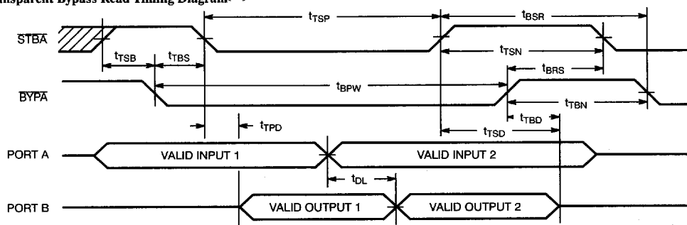
Transparent Bypass Read Timing Diagram [14]
