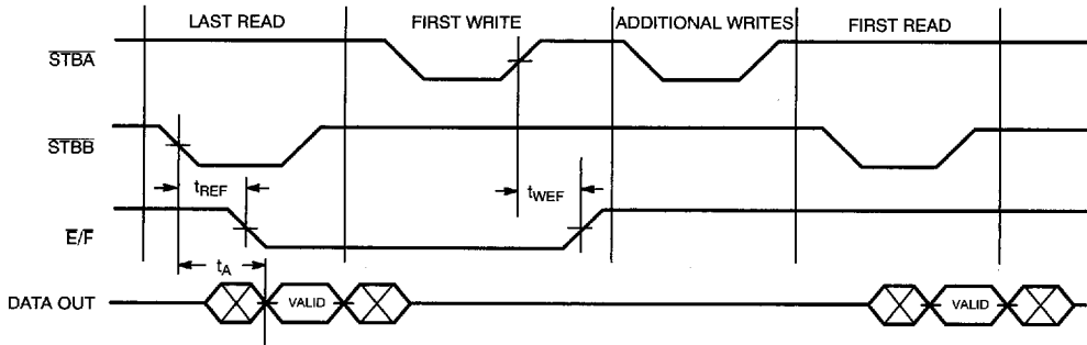
Empty/Full Flag and Read Bubble-Through Mode Timing Diagram [11]
