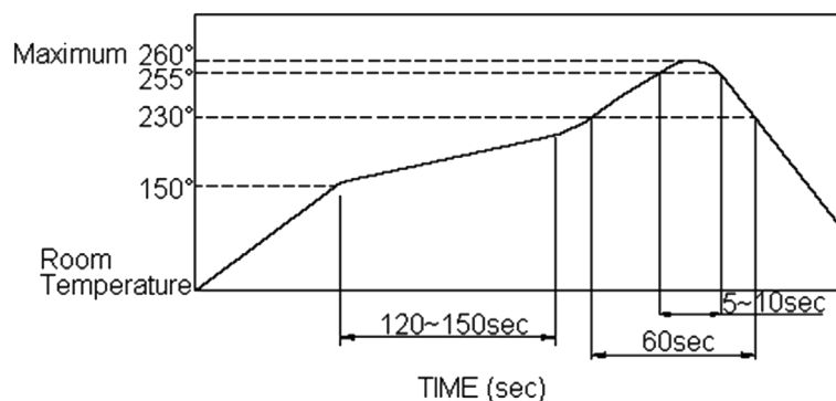
Reflow Temperature Profile
