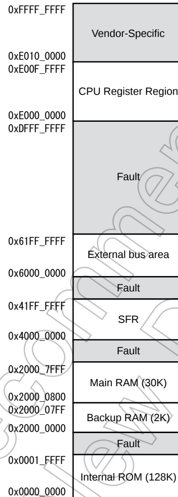
Figure 4-3 Memory Map (TMPM366FW)
