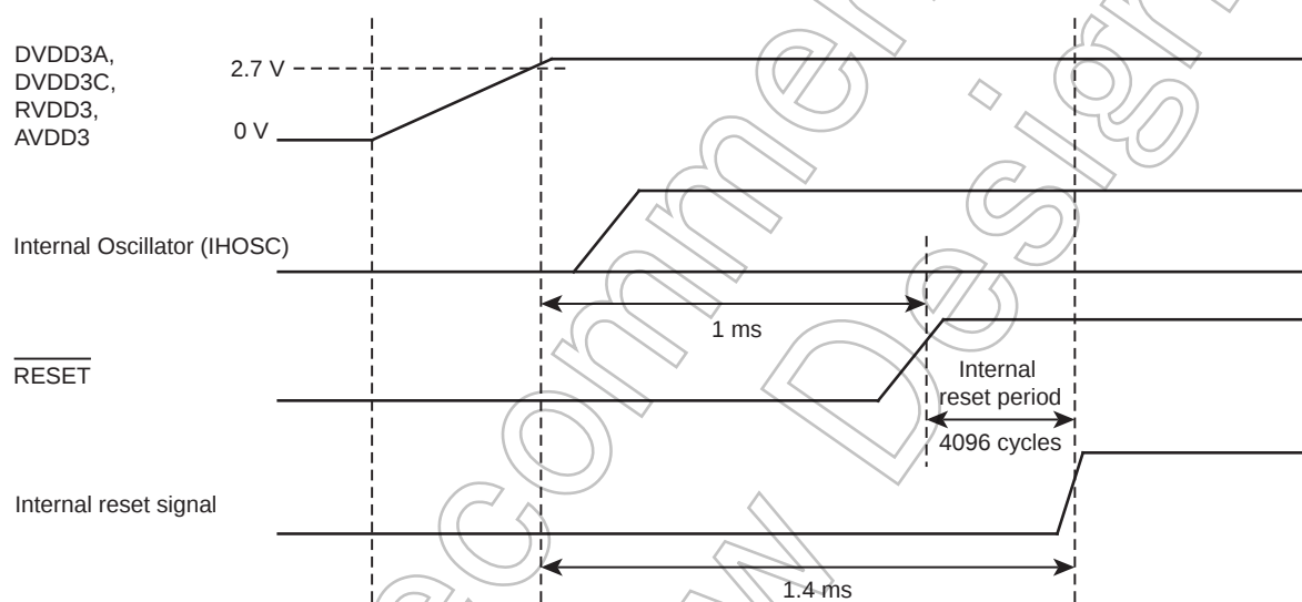
Figure 22-2 Power-on sequence
