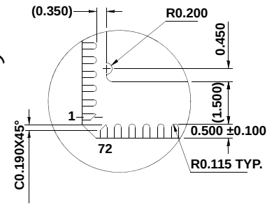
DETAIL "Z"
