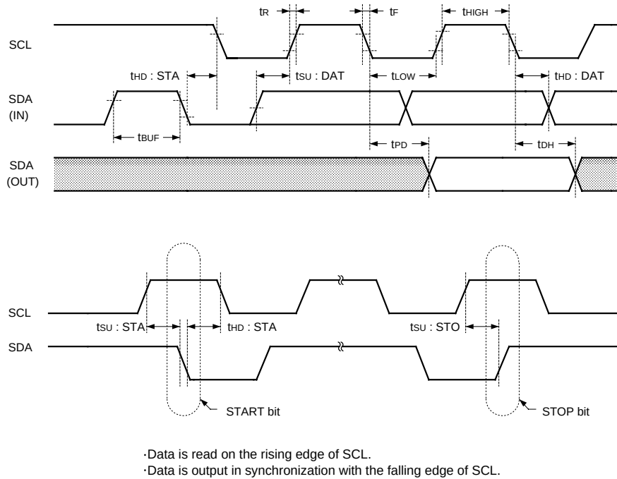
Fig.1 Synchronized data input / output timing
