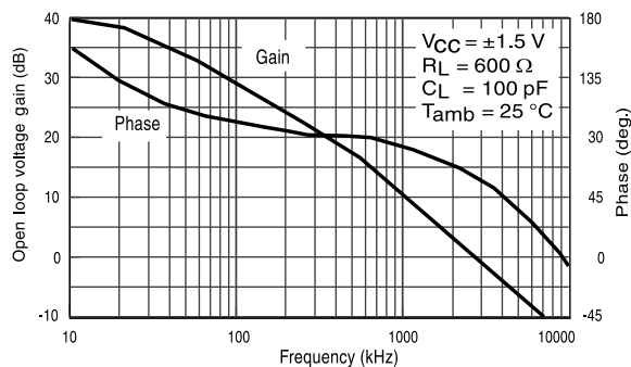
Figure 3. Voltage gain and phase vs. frequency
