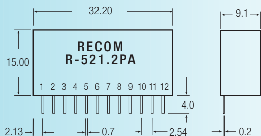
SIP12 PIN Package
