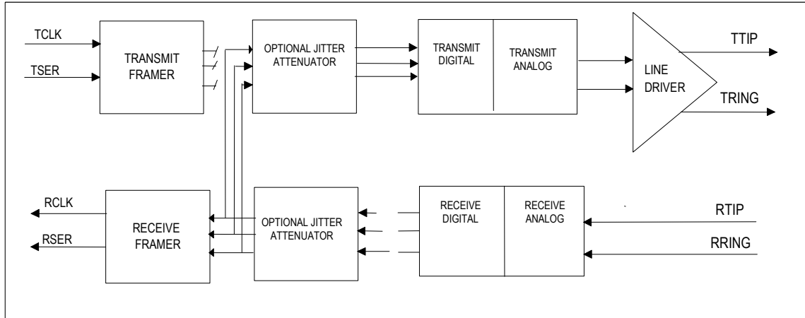
Figure 8-18. Remote Loopback
