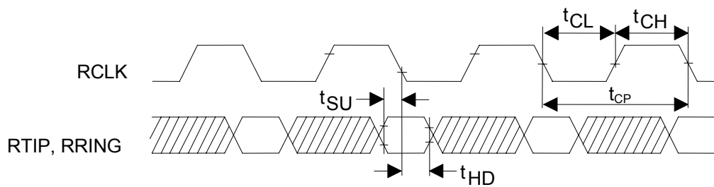
Figure 12-7. Receive Framing Timing—Line Side
