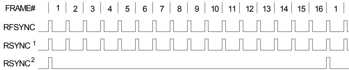
Figure 10-15. E1 Receive-Side Timing
