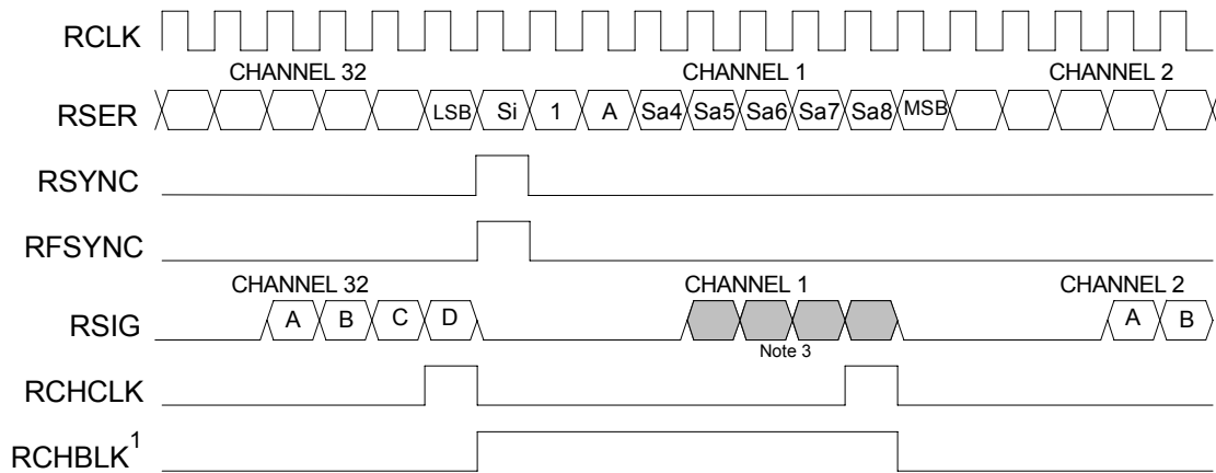
Figure 10-16. E1 Receive-Side Boundary Timing (Elastic Store Disabled)
