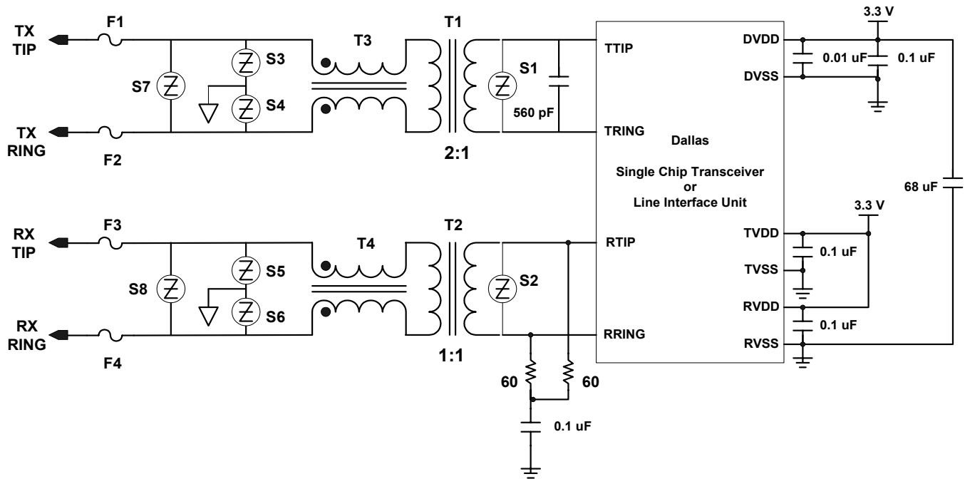
Figure 8-11. Network Connection for Software-Selected Termination—Longitudinal Protection
