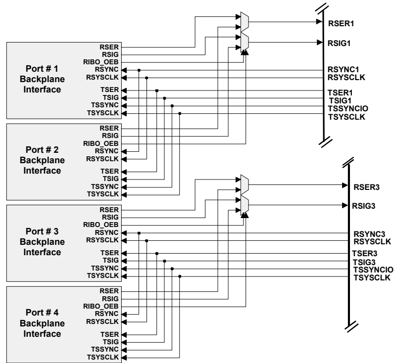
Figure 8-3. IBO Multiplexer Equivalent Circuit—4.096MHz
