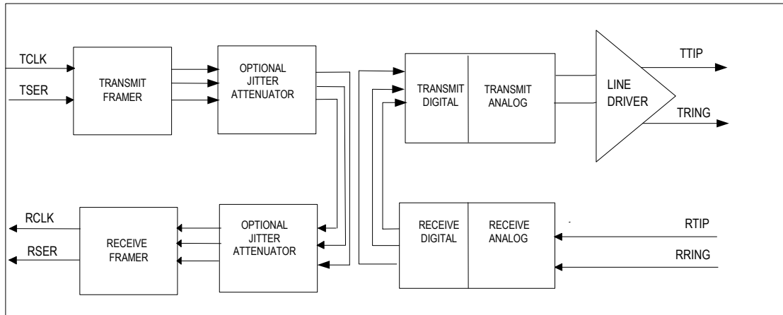
Figure 8-19. Dual Loopback
