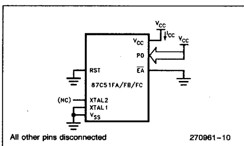
Figure 9. I_{CC} Test Condition, Power Down Mode. V_{CC} = 2.0V to 5.5V .
